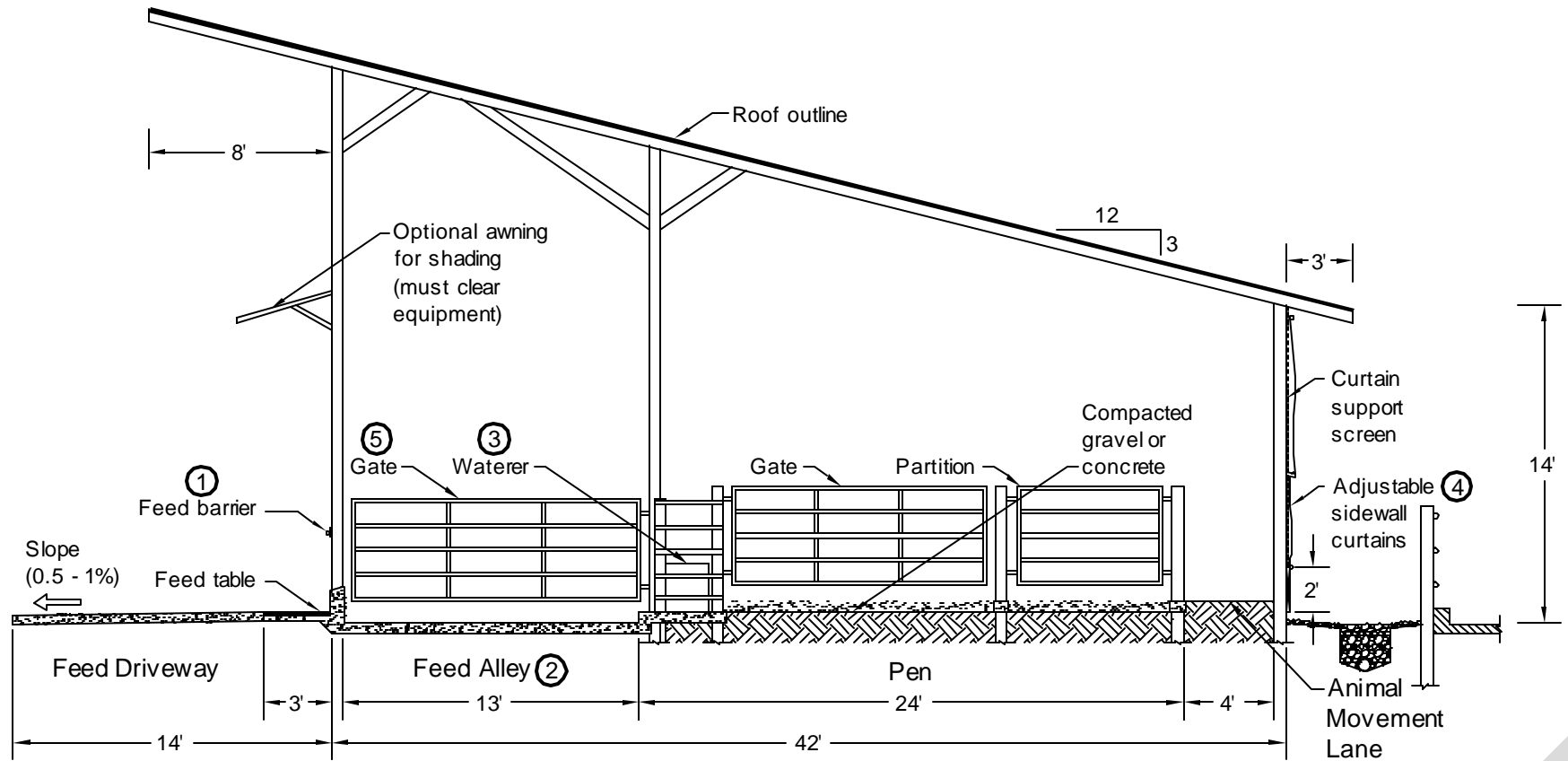
Monoslope Roof (1) Cross Section (2)
