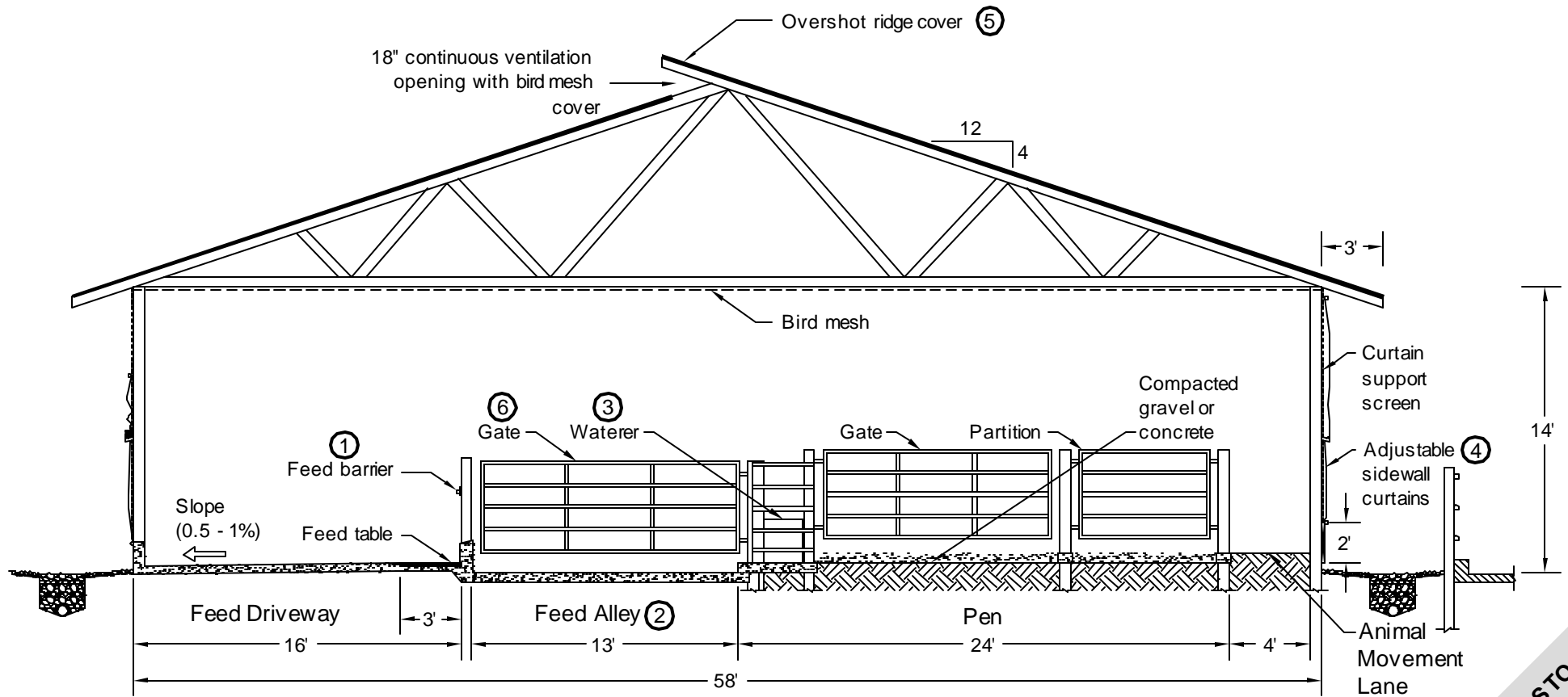
Gable Roof Cross Section, Inside Feeding
