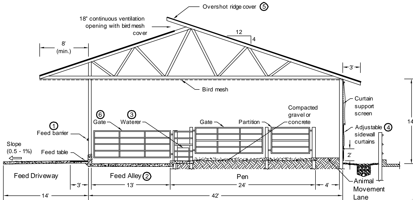
Gable Roof (1) Cross Section (3)
